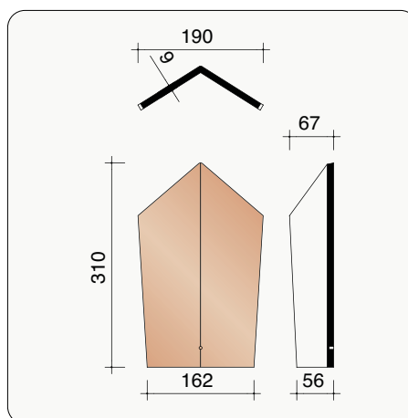
P0003711 About de cornier
